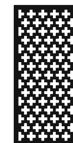
Algebra
