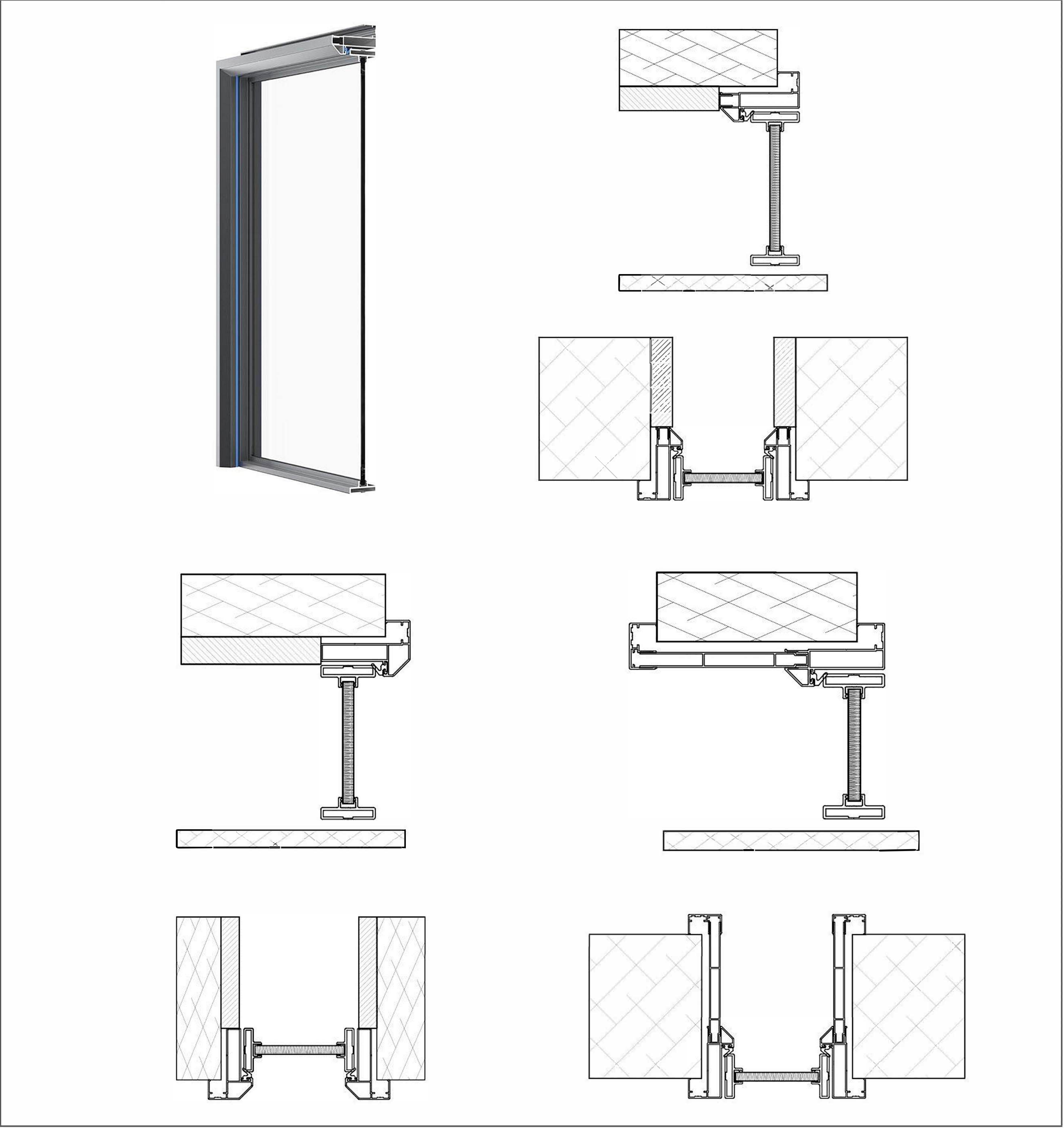
Model: YT-OPJZ99B-X Thickness: 1.0mm Name: * Weight: 0.280kg/m
