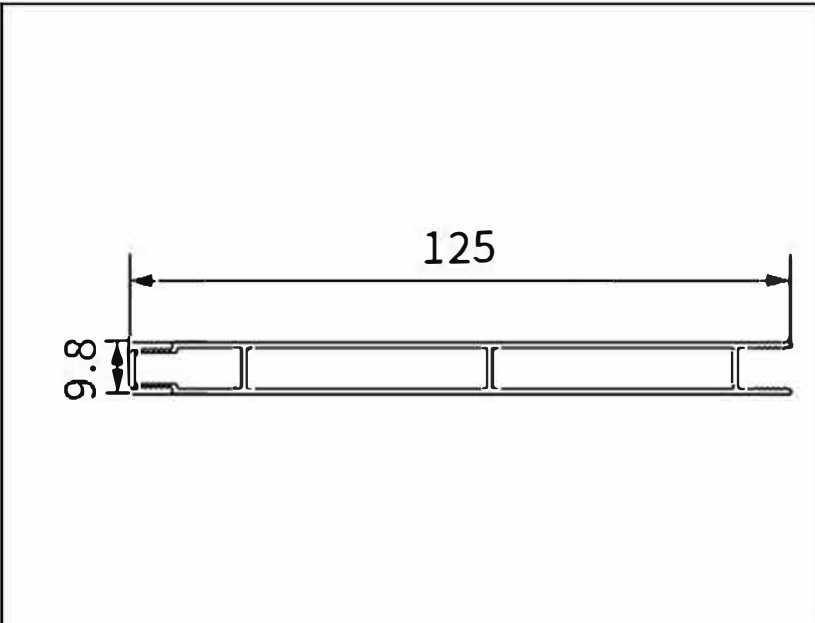
Model: YT-Z80180B-L Thickness: 1.0mm Name: * Weight: 0.75kg/m
