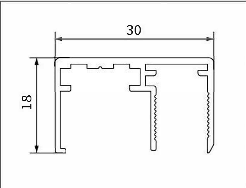
Model: YT-OPJZ99B-X Thickness: 1.0mm Name: * Weight: 0.280kg/m
