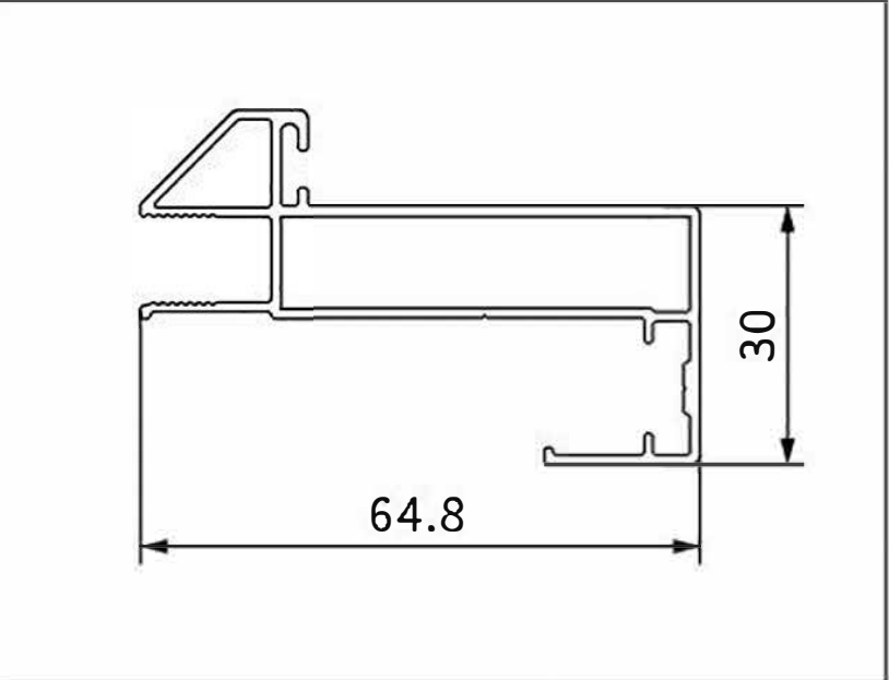
Model: YT-OPJZ101B-L Thickness: 1.1mm Name: * Weight: 0.720kg/m
