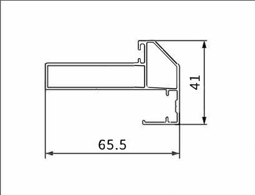
Model: YT-OPJZ100B-L Thickness: 1.1mm Name: * Weight: 0.716kg/m
