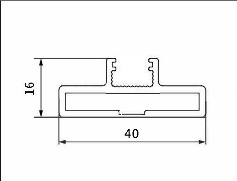
Model: YT-OPJZ97B-X Thickness: 1.8mm Name: * Weight: 0.508kg/m
