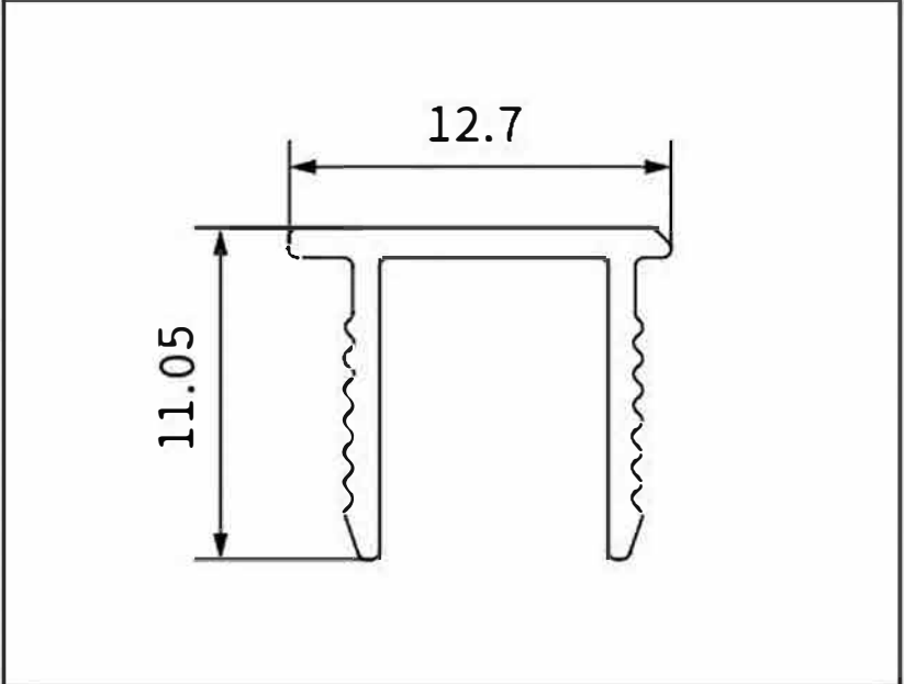
Model: YT-OPJZ98B-S Thickness: 1.15mm Name: * Weight: 0.087kg/m
