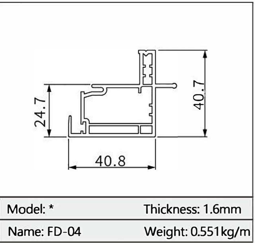
HUNG WINDOW
